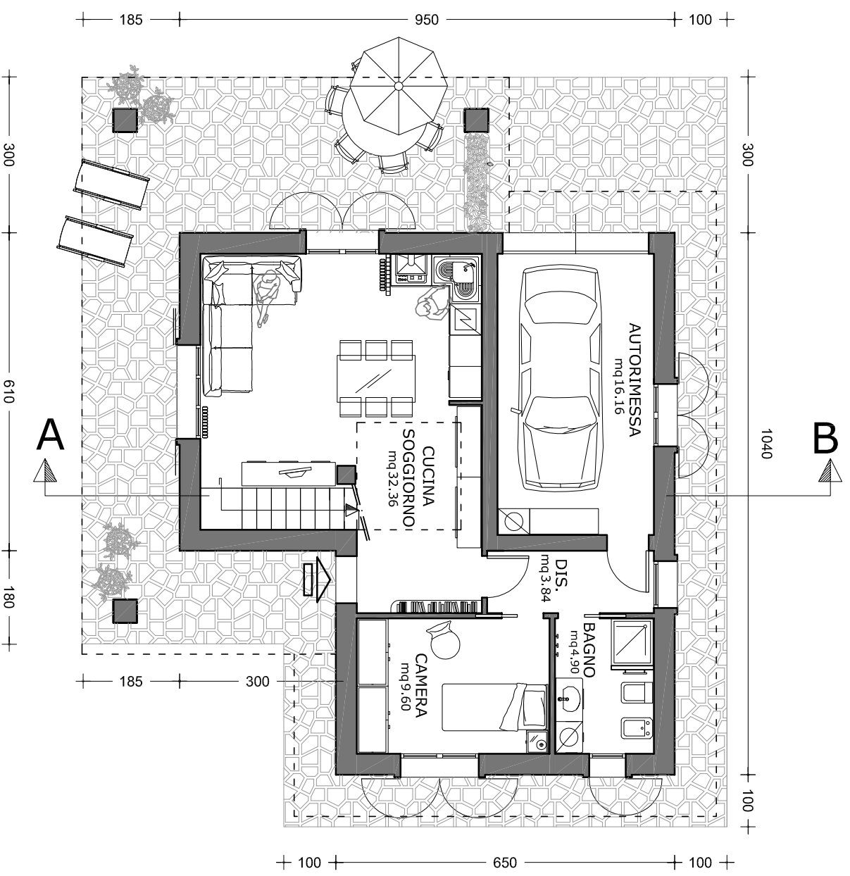
PIANO TERRA
